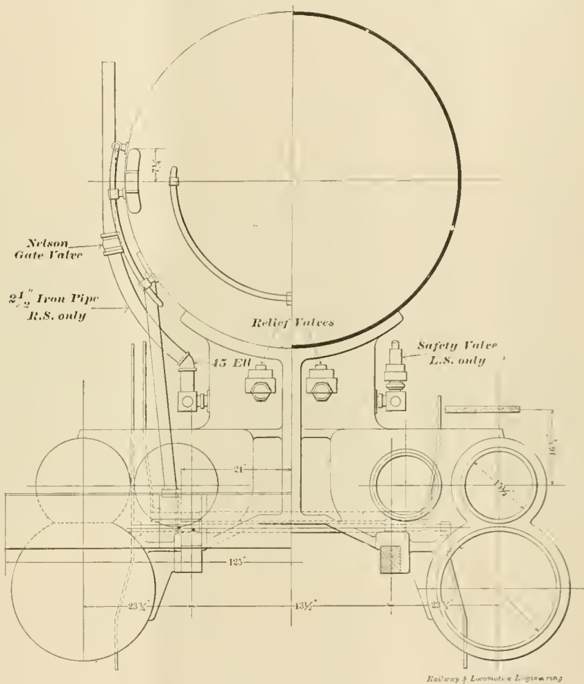
BALDWIN BACK PRESSURE BRAKE—NORTHERN PACIFIC.
